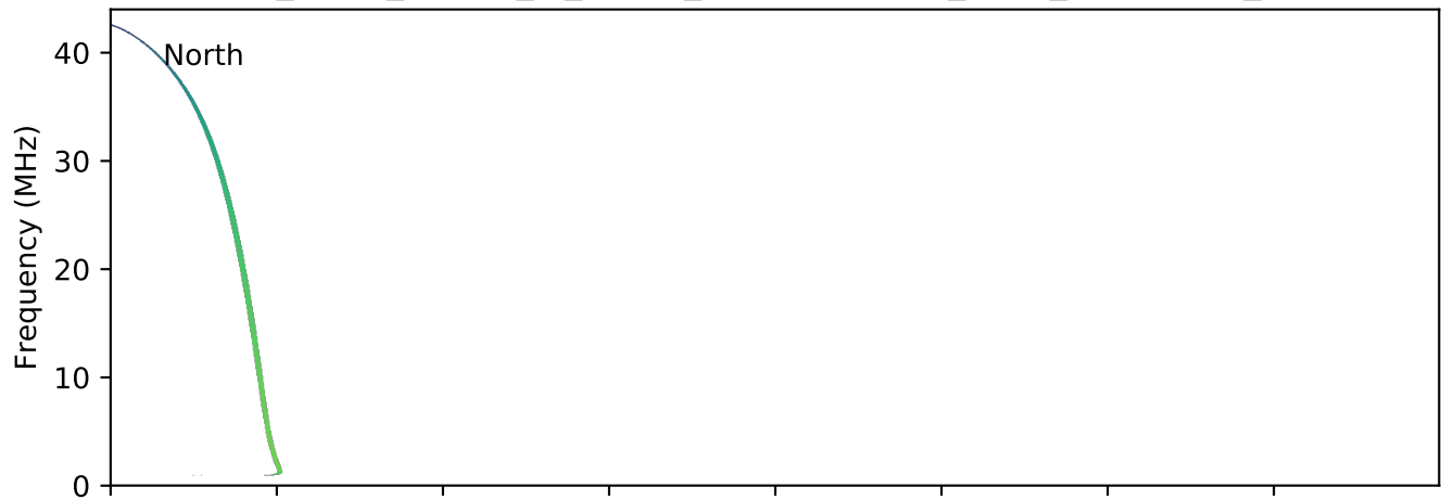
expres_earth_jupiter_io_jrm09_lossc-wid1deg_3kev_20090708_v01.cdf
