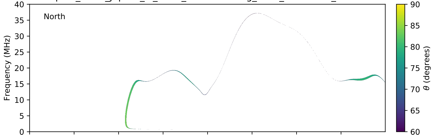
expres_earth_jupiter_io_isaac_lossc-wid1deg_3kev_20090730_v01.cdf
