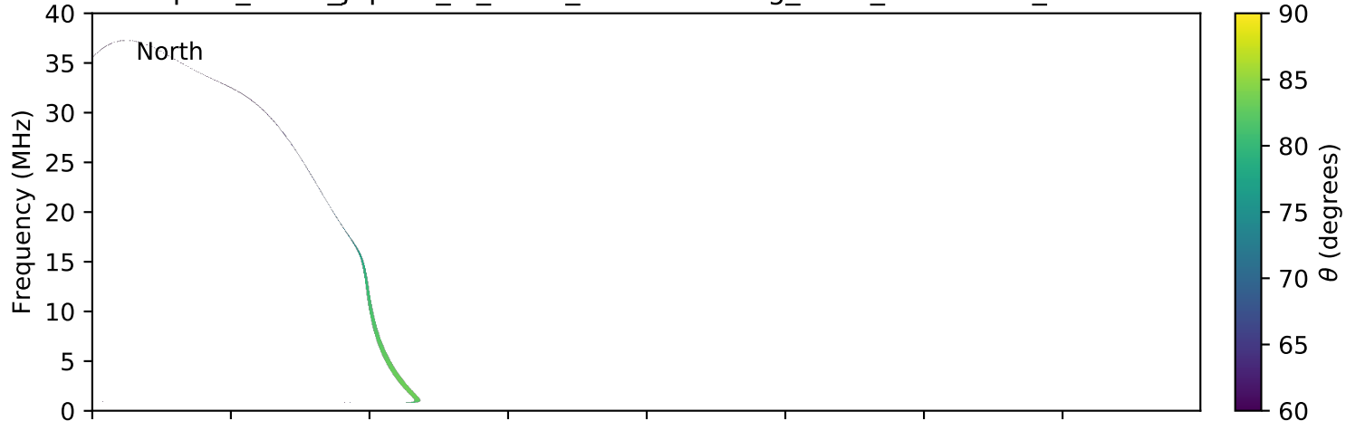
expres_earth_jupiter_io_isaac_lossc-wid1deg_3kev_20090729_v01.cdf
