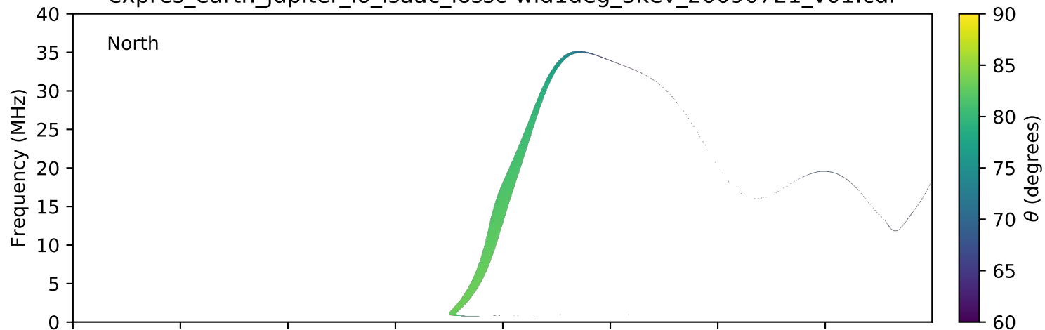
expres_earth_jupiter_io_isaac_lossc-wid1deg_3kev_20090721_v01.cdf
