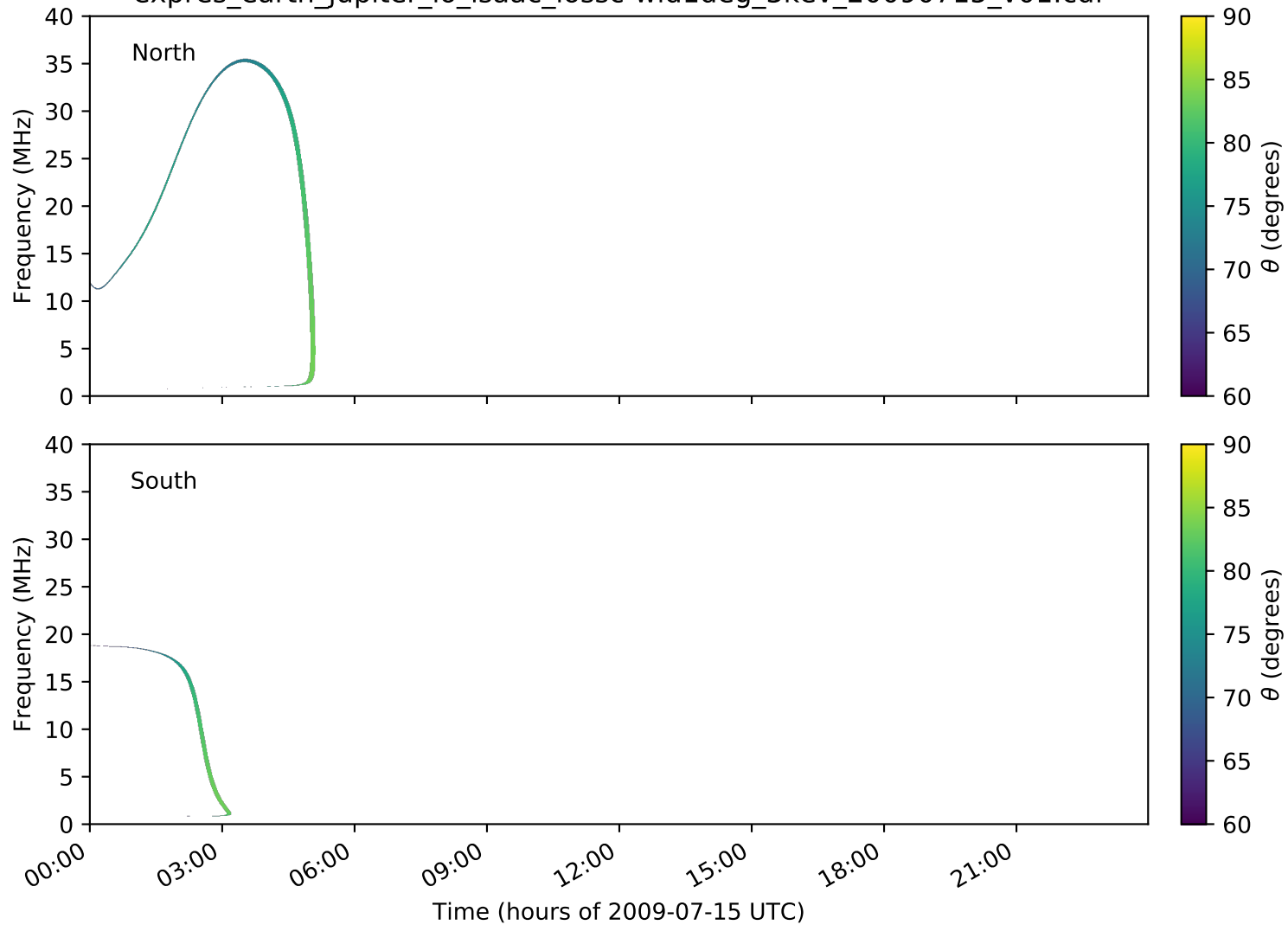
expres_earth_jupiter_io_isaac_lossc-wid1deg_3kev_20090715_v01.cdf
