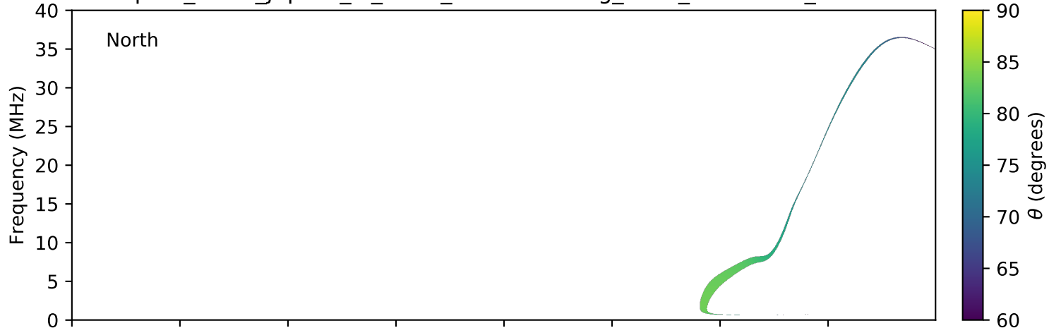
expres_earth_jupiter_io_isaac_lossc-wid1deg_3kev_20090703_v01.cdf
