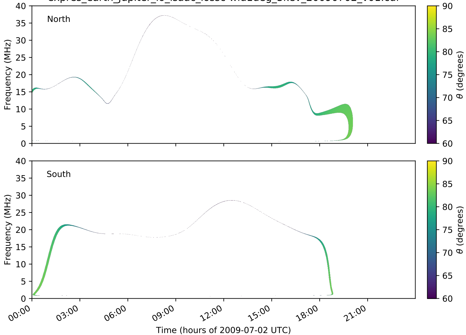
expres_earth_jupiter_io_isaac_lossc-wid1deg_3kev_20090702_v01.cdf
