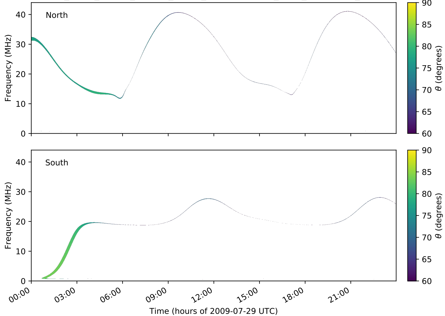
expres_earth_jupiter_europa_jrm09_lossc-wid1deg_3kev_20090729_v01.cdf
