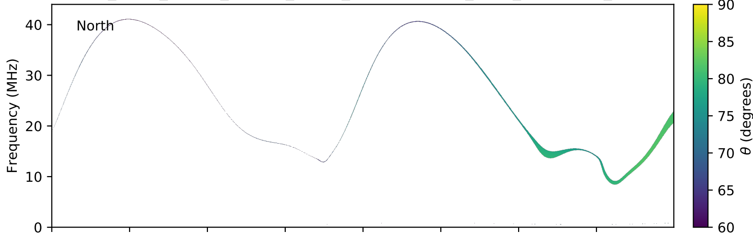
expres_earth_jupiter_europa_jrm09_lossc-wid1deg_3kev_20090726_v01.cdf
