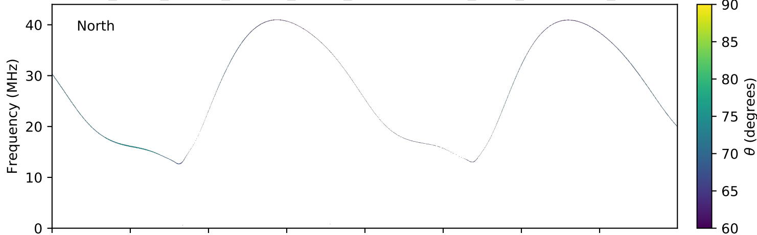
expres_earth_jupiter_europa_jrm09_lossc-wid1deg_3kev_20090715_v01.cdf
