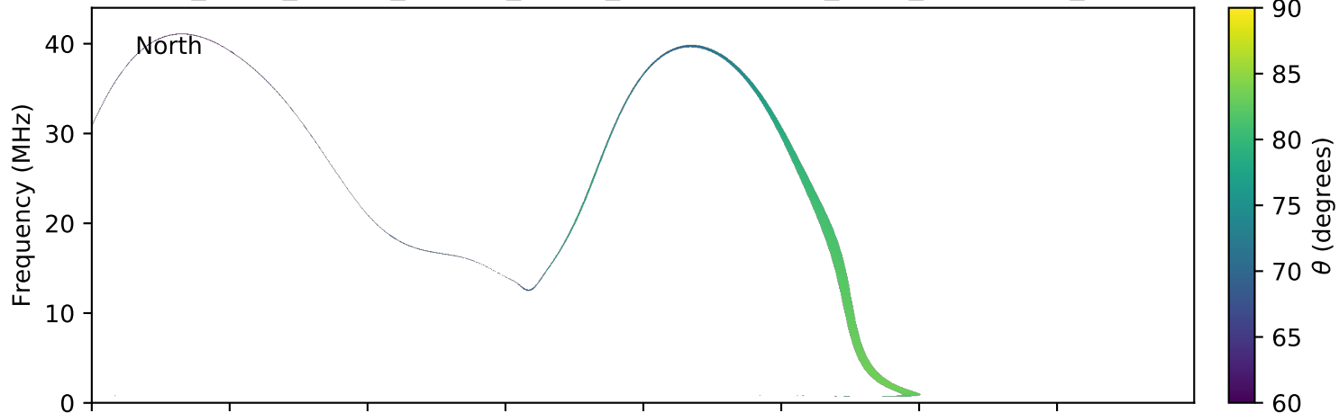
expres_earth_jupiter_europa_jrm09_lossc-wid1deg_3kev_20090712_v01.cdf
