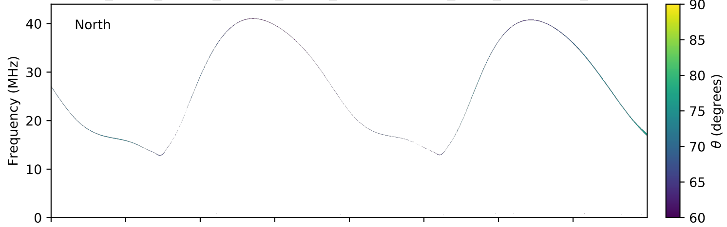
expres_earth_jupiter_europa_jrm09_lossc-wid1deg_3kev_20090708_v01.cdf
