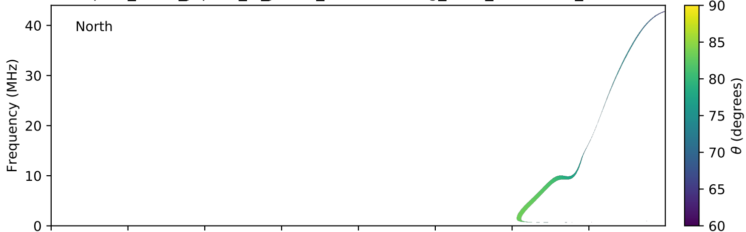
expres_earth_jupiter_io_jrm09_lossc-wid1deg_3kev_20090610_v01.cdf
