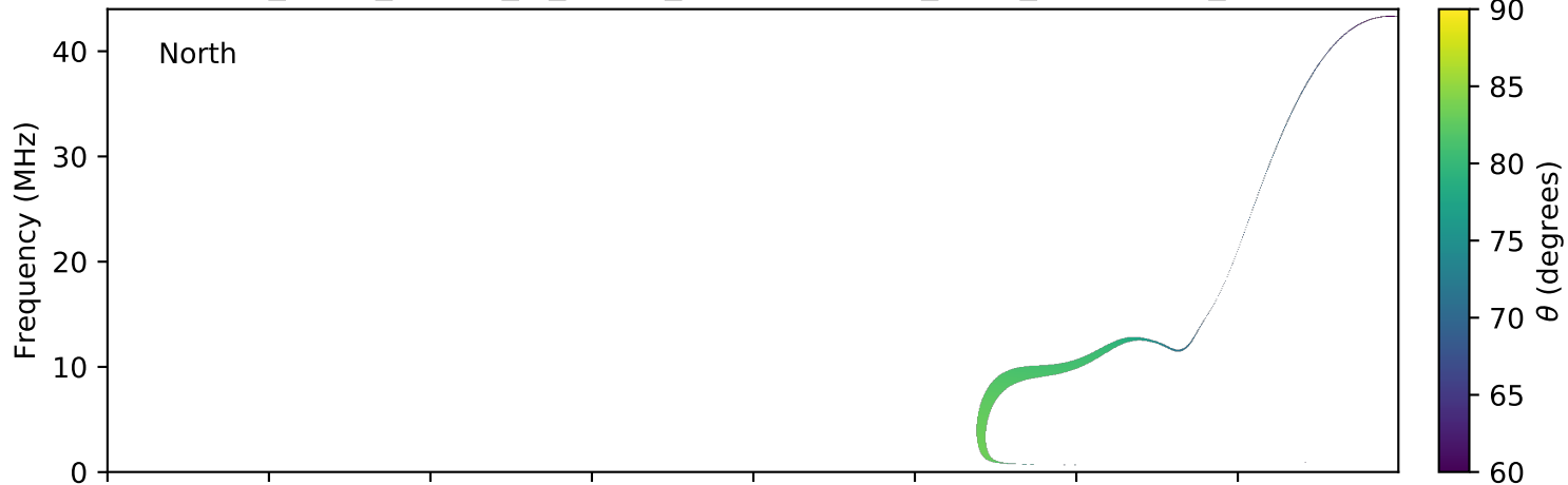
expres_earth_jupiter_io_jrm09_lossc-wid1deg_3kev_20090603_v01.cdf
