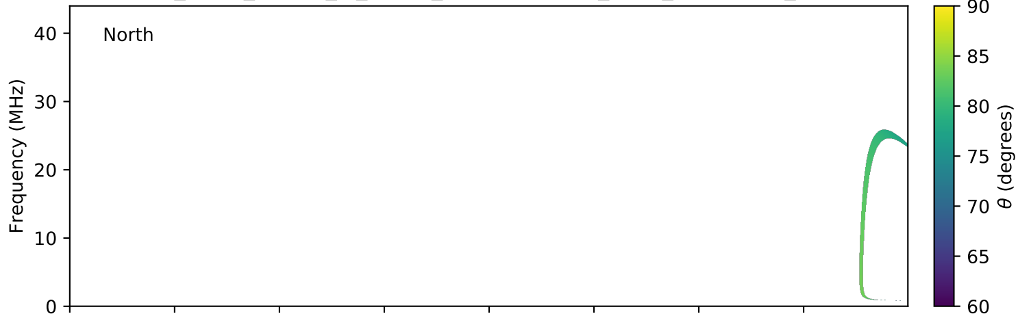
expres_earth_jupiter_io_jrm09_lossc-wid1deg_3kev_20090601_v01.cdf
