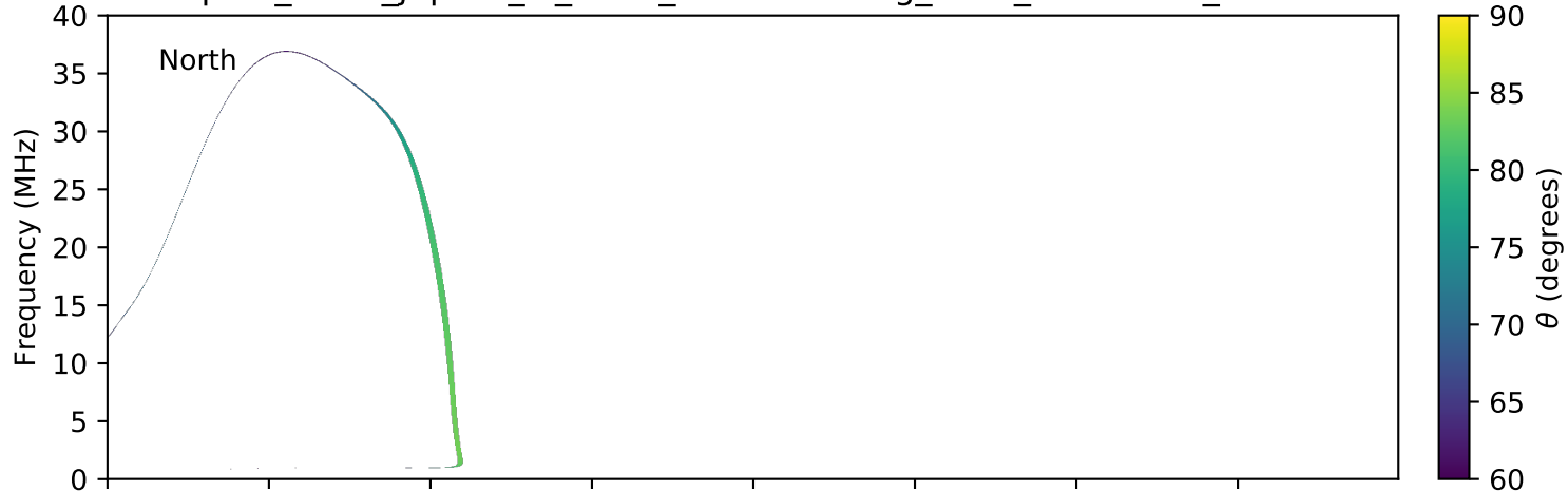
expres_earth_jupiter_io_isaac_lossc-wid1deg_3kev_20090629_v01.cdf
