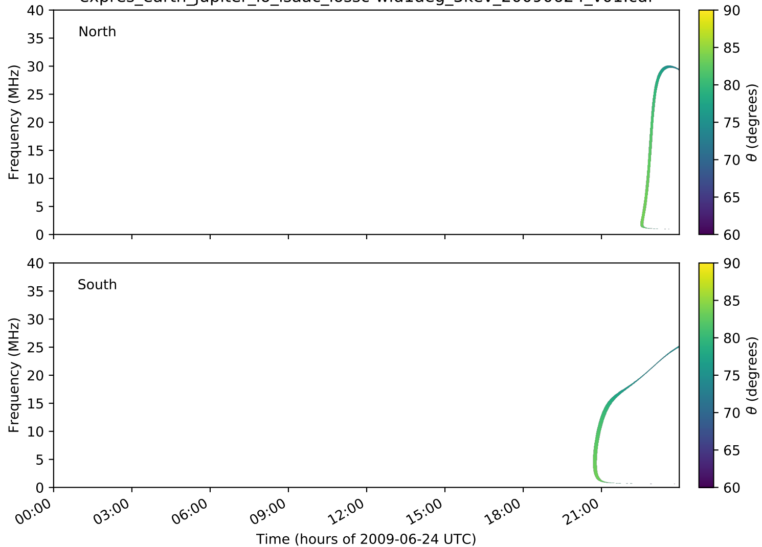
expres_earth_jupiter_io_isaac_lossc-wid1deg_3kev_20090624_v01.cdf
