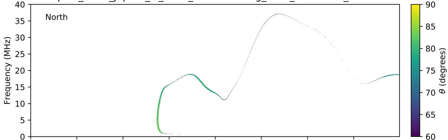
expres_earth_jupiter_io_isaac_lossc-wid1deg_3kev_20090621_v01.cdf
