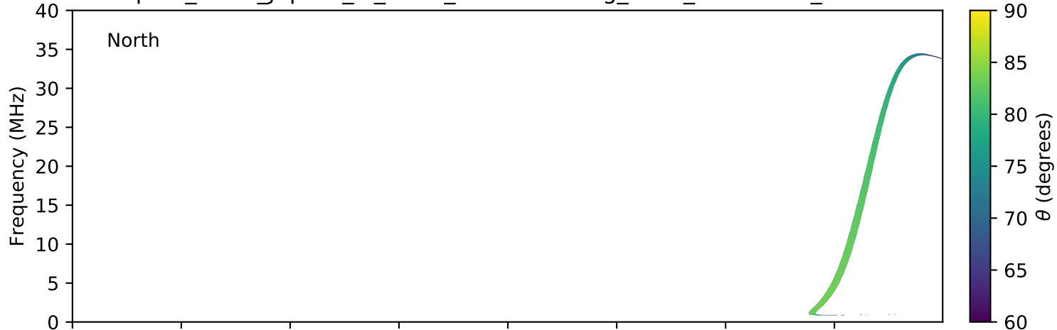
expres_earth_jupiter_io_isaac_lossc-wid1deg_3kev_20090617_v01.cdf
