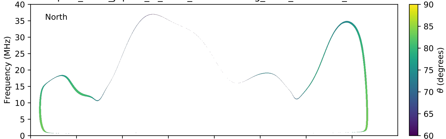
expres_earth_jupiter_io_isaac_lossc-wid1deg_3kev_20090616_v01.cdf
