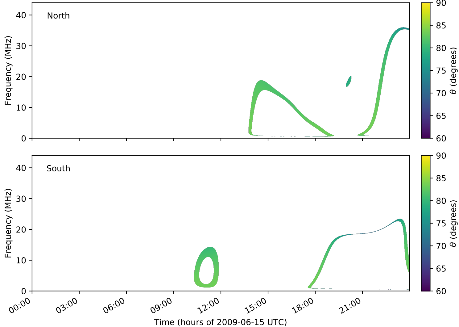
expres_earth_jupiter_ganymede_jrm09_lossc-wid1deg_3kev_20090615_v01.cdf
