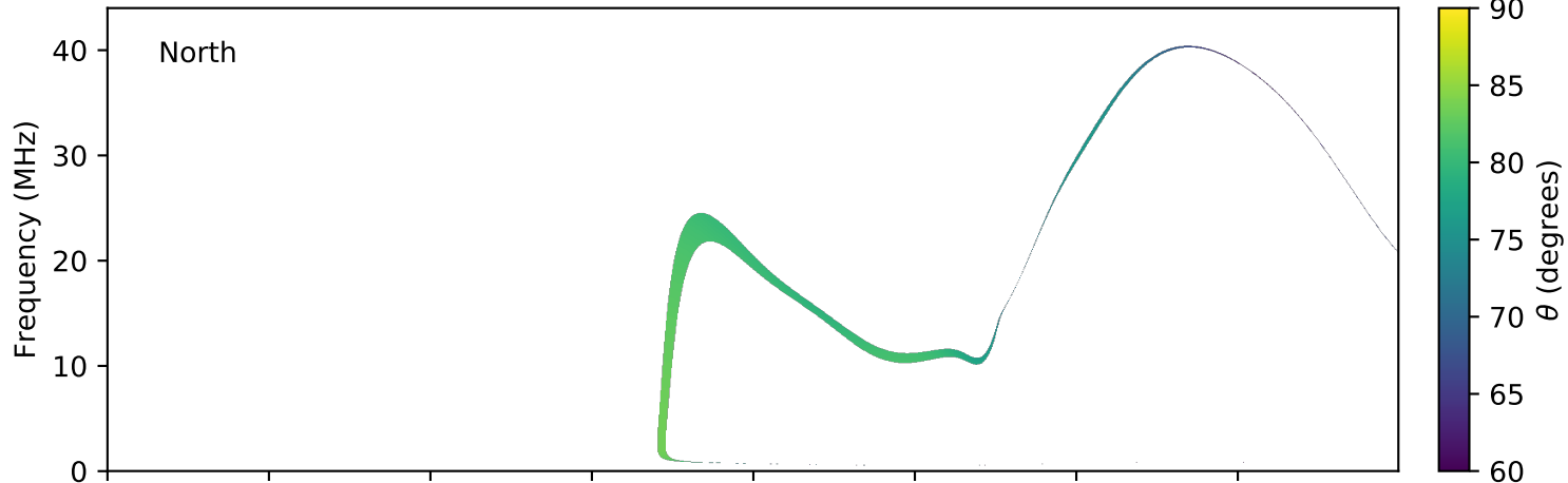
expres_earth_jupiter_europa_jrm09_lossc-wid1deg_3kev_20090623_v01.cdf
