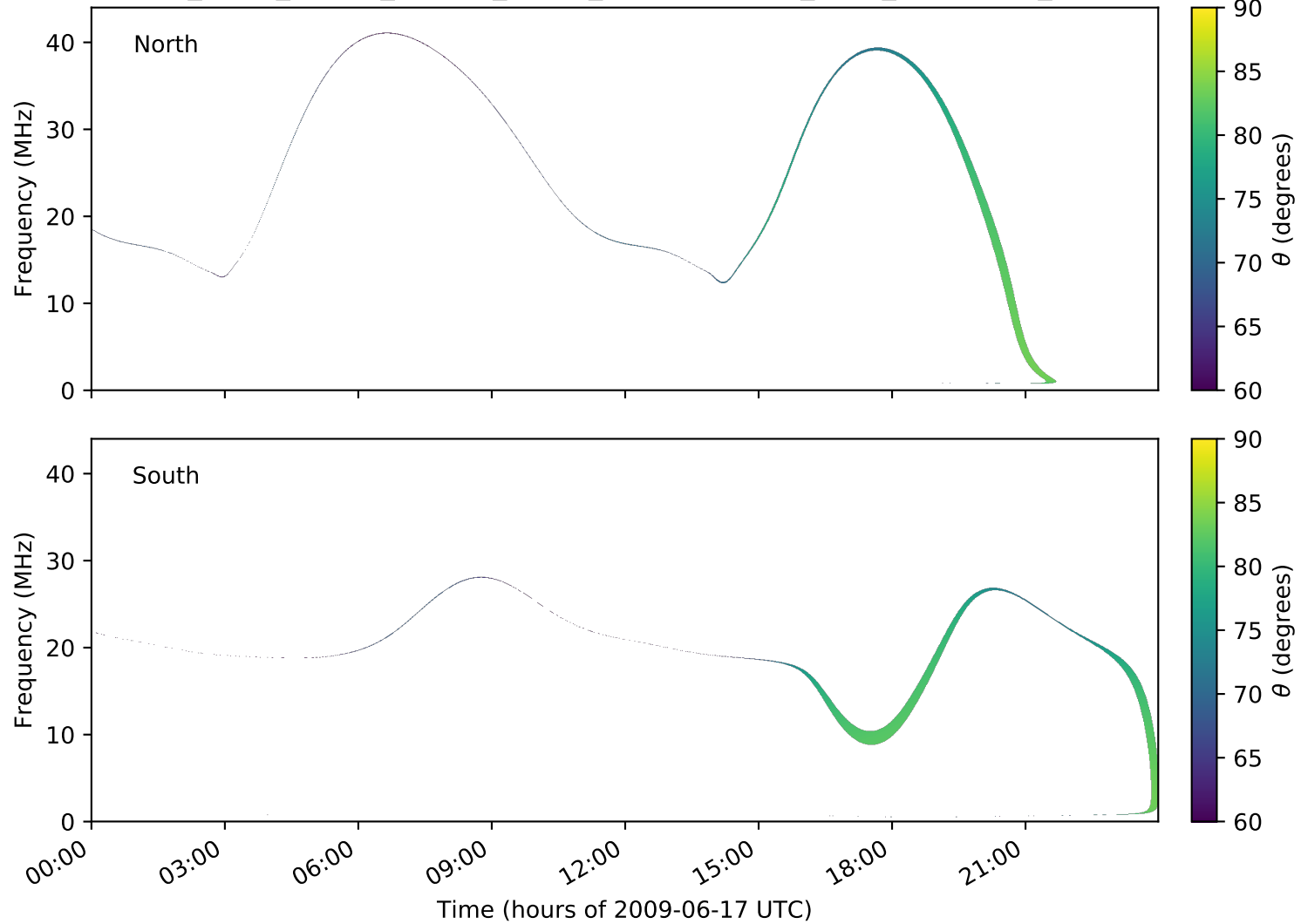
expres_earth_jupiter_europa_jrm09_lossc-wid1deg_3kev_20090617_v01.cdf
