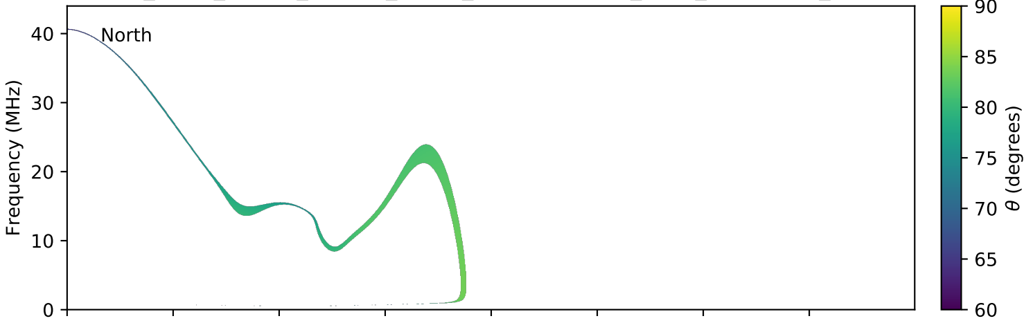
expres_earth_jupiter_europa_jrm09_lossc-wid1deg_3kev_20090614_v01.cdf
