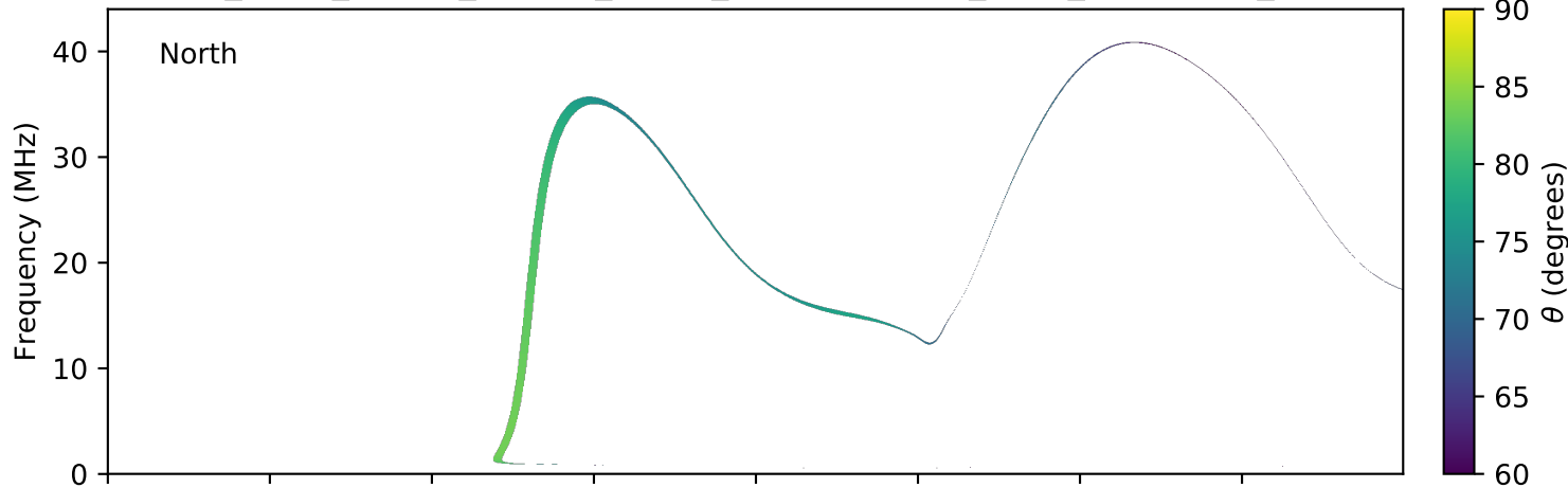
expres_earth_jupiter_europa_jrm09_lossc-wid1deg_3kev_20090609_v01.cdf
