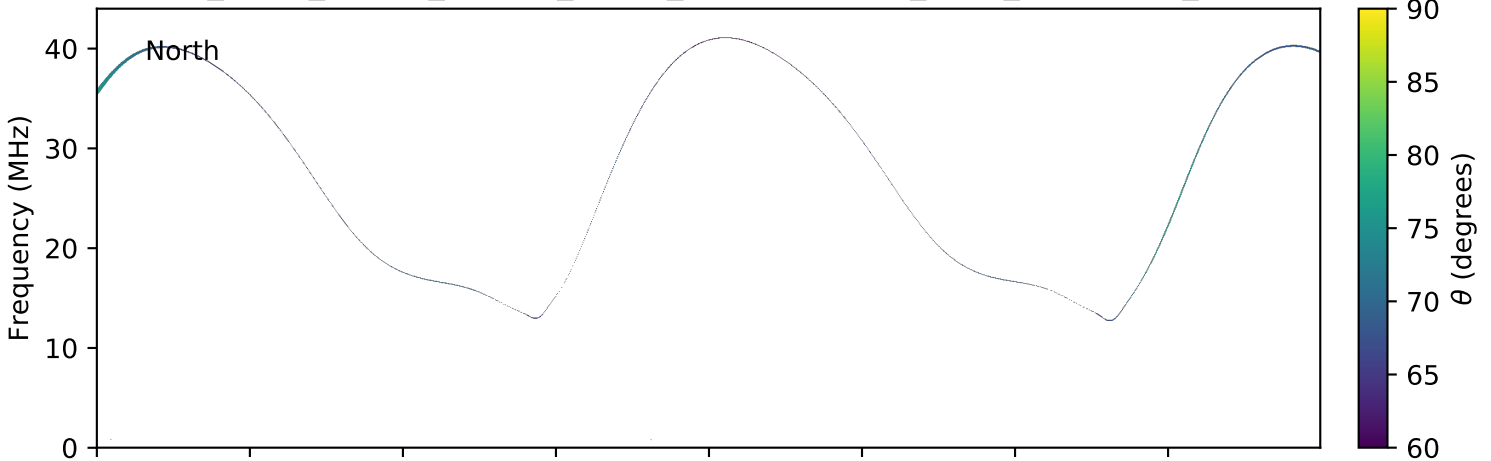
expres_earth_jupiter_europa_jrm09_lossc-wid1deg_3kev_20090606_v01.cdf
