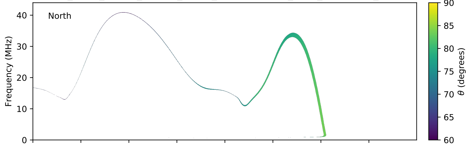
expres_earth_jupiter_europa_jrm09_lossc-wid1deg_3kev_20090603_v01.cdf
