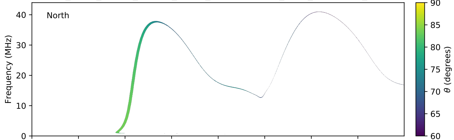
expres_earth_jupiter_europa_jrm09_lossc-wid1deg_3kev_20090602_v01.cdf
