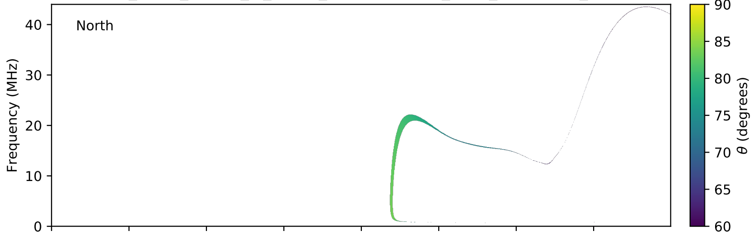
expres_earth_jupiter_io_jrm09_lossc-wid1deg_3kev_20090520_v01.cdf
