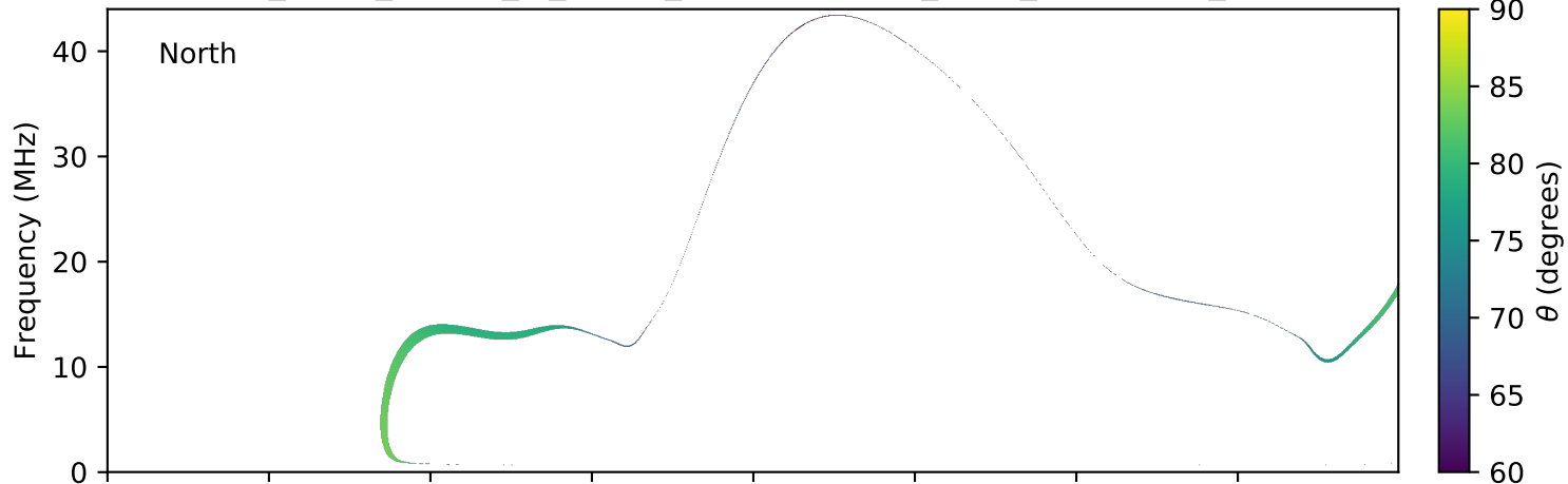
expres_earth_jupiter_io_jrm09_lossc-wid1deg_3kev_20090515_v01.cdf
