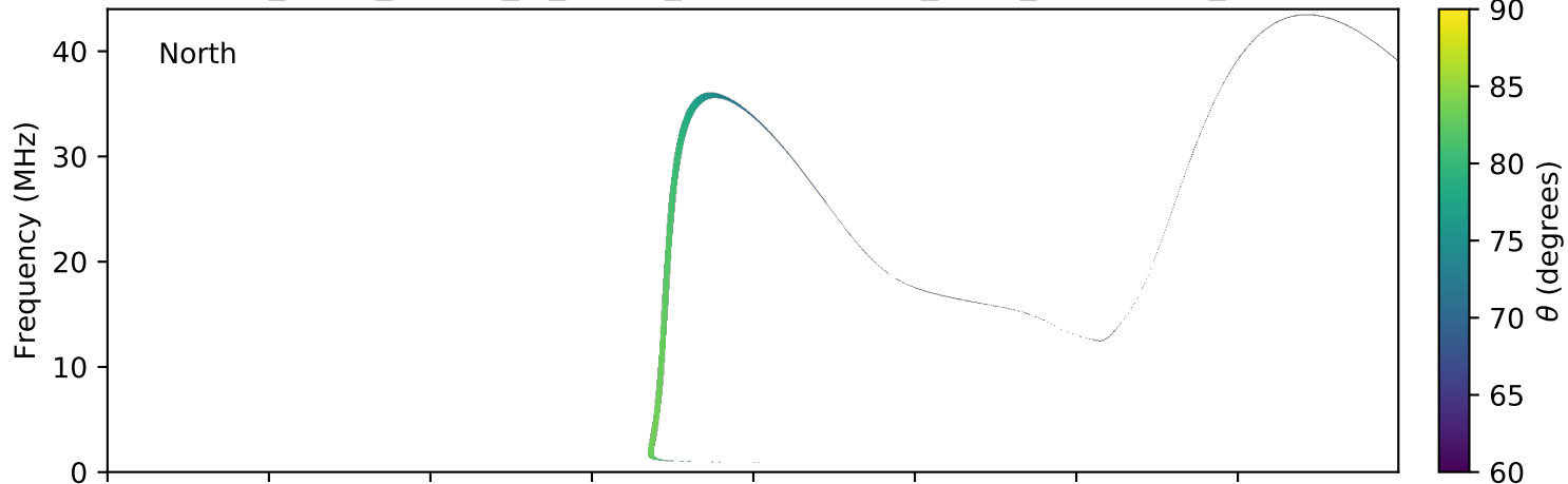
expres_earth_jupiter_io_jrm09_lossc-wid1deg_3kev_20090506_v01.cdf
