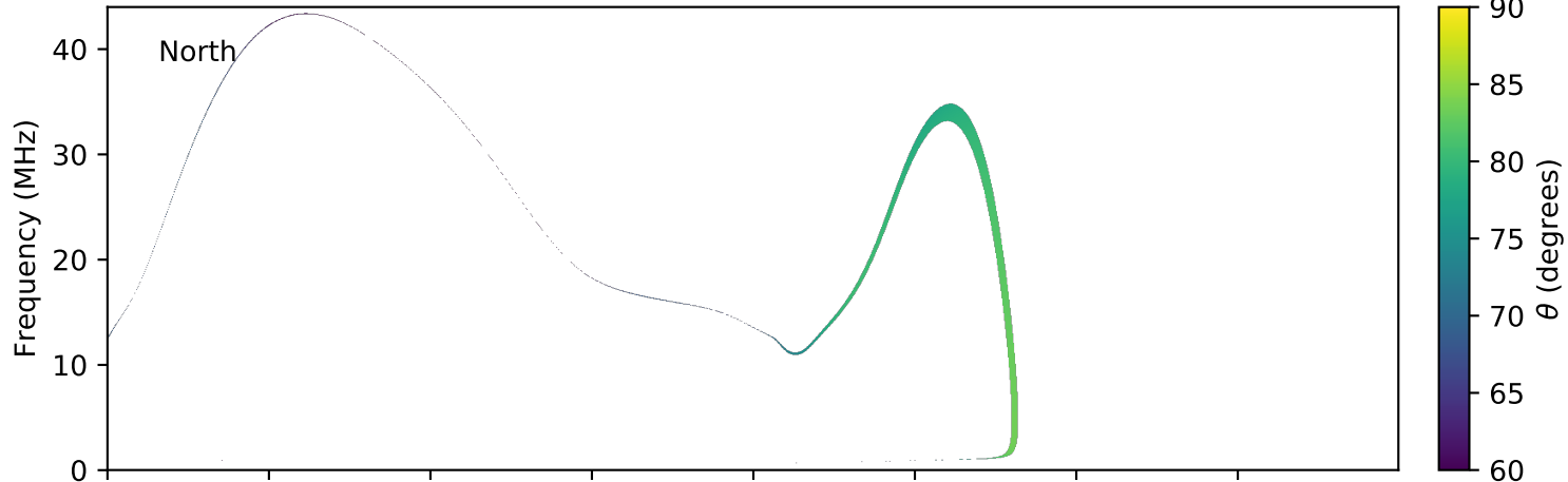
expres_earth_jupiter_io_jrm09_lossc-wid1deg_3kev_20090503_v01.cdf
