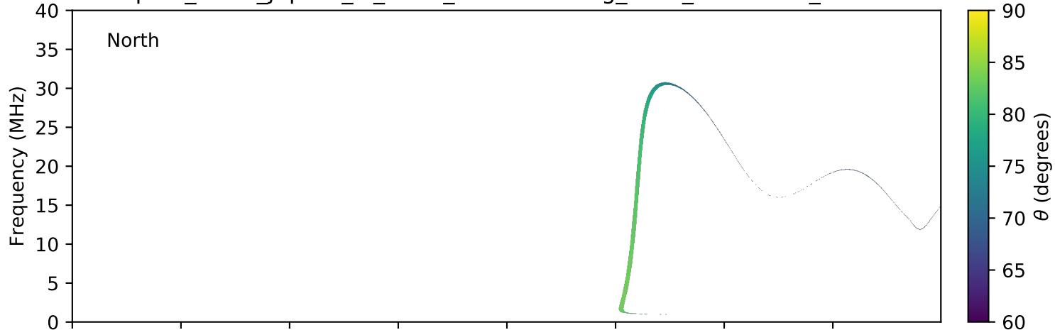
expres_earth_jupiter_io_isaac_lossc-wid1deg_3kev_20090527_v01.cdf
