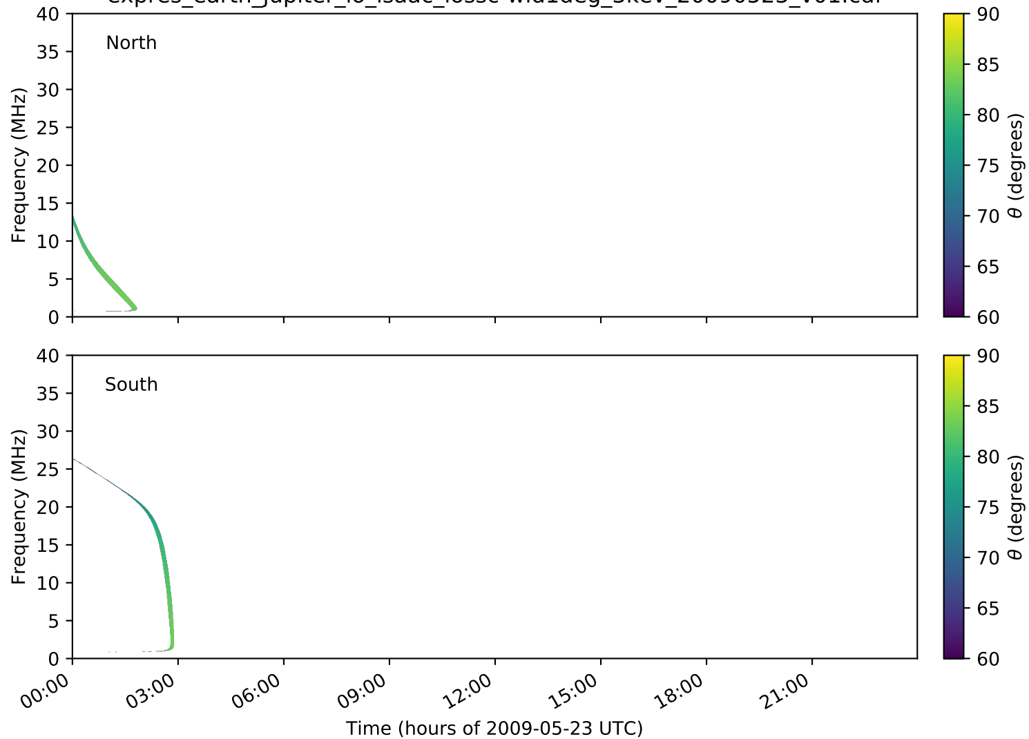
expres_earth_jupiter_io_isaac_lossc-wid1deg_3kev_20090523_v01.cdf
