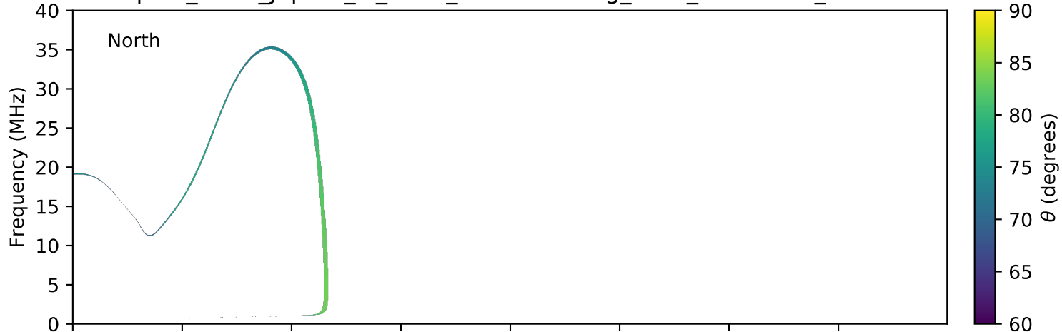
expres_earth_jupiter_io_isaac_lossc-wid1deg_3kev_20090514_v01.cdf
