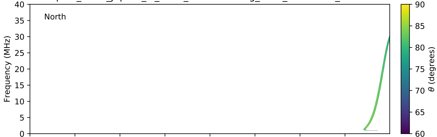
expres_earth_jupiter_io_isaac_lossc-wid1deg_3kev_20090509_v01.cdf
