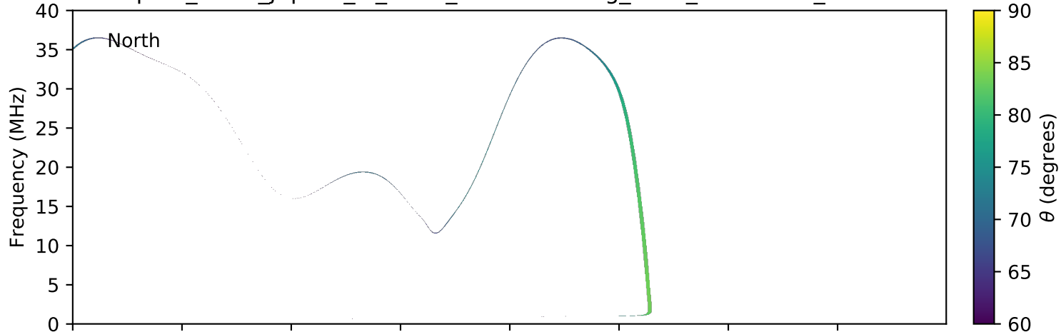
expres_earth_jupiter_io_isaac_lossc-wid1deg_3kev_20090503_v01.cdf
