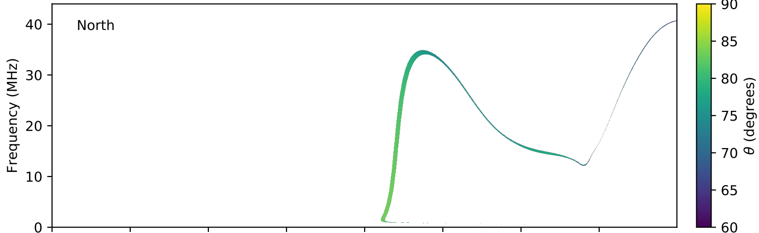
expres_earth_jupiter_europa_jrm09_lossc-wid1deg_3kev_20090522_v01.cdf
