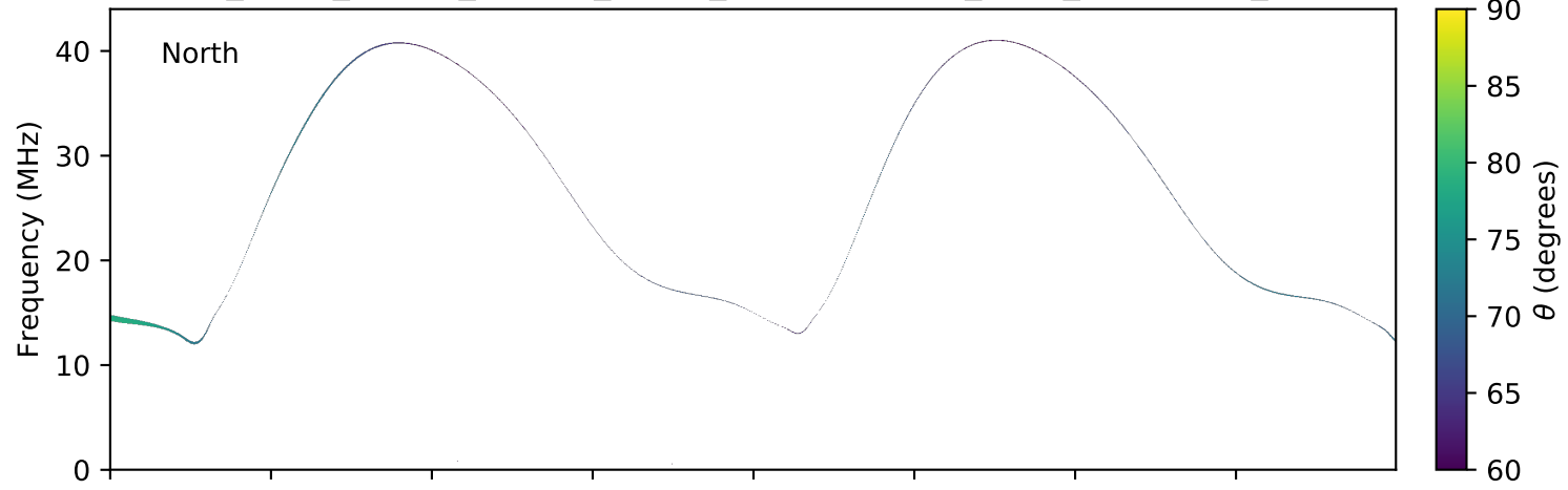
expres_earth_jupiter_europa_jrm09_lossc-wid1deg_3kev_20090505_v01.cdf
