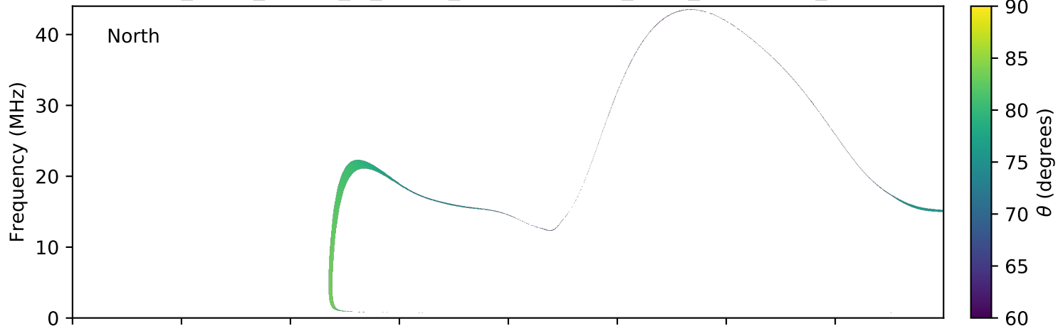
expres_earth_jupiter_io_jrm09_lossc-wid1deg_3kev_20090406_v01.cdf
