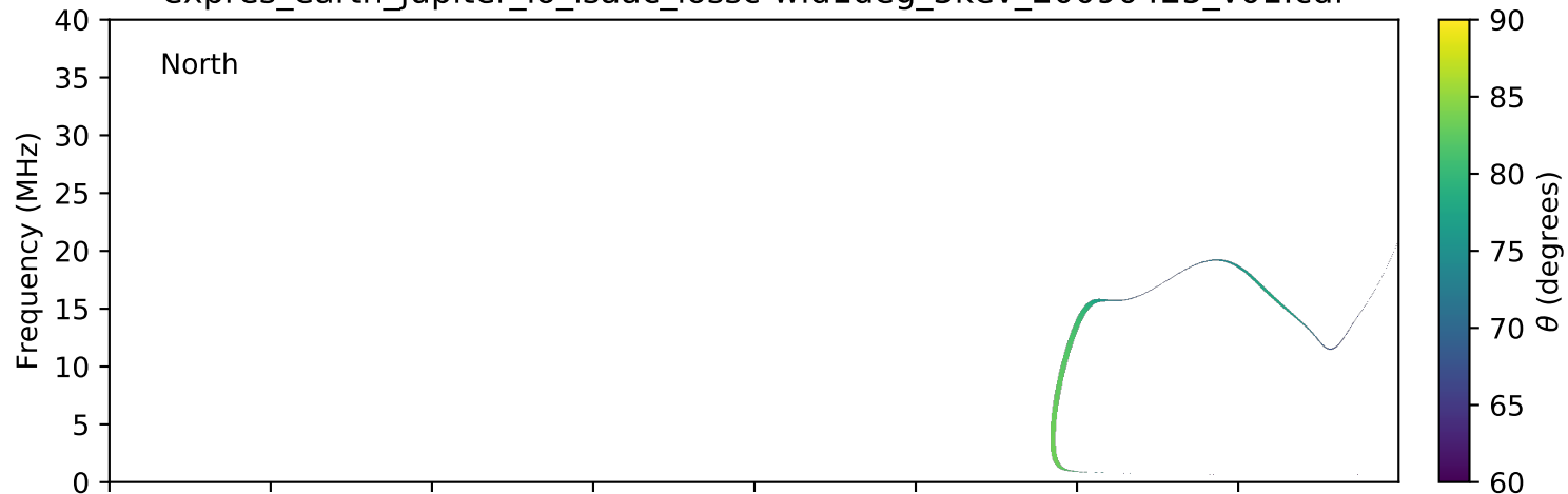
expres_earth_jupiter_io_isaac_lossc-wid1deg_3kev_20090425_v01.cdf
