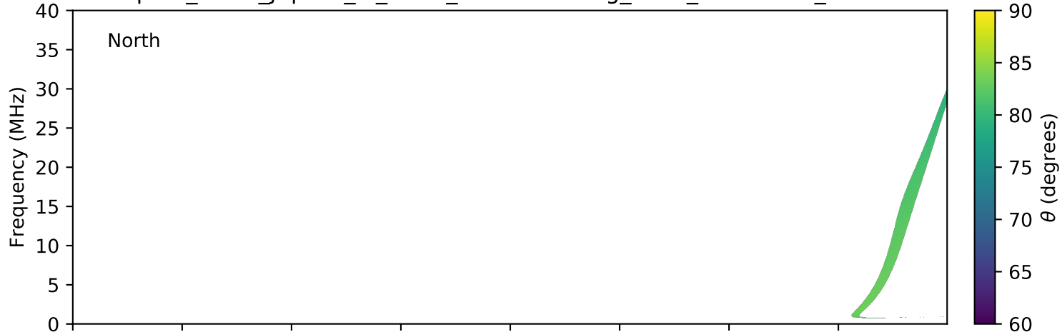
expres_earth_jupiter_io_isaac_lossc-wid1deg_3kev_20090416_v01.cdf
