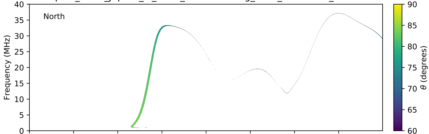
expres_earth_jupiter_io_isaac_lossc-wid1deg_3kev_20090406_v01.cdf
