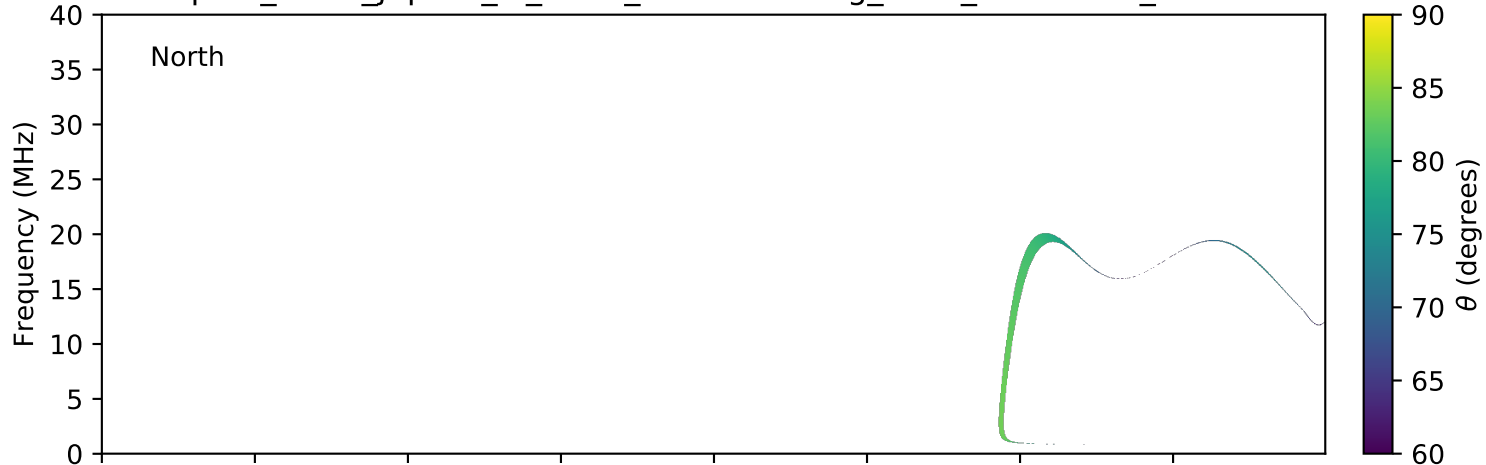
expres_earth_jupiter_io_isaac_lossc-wid1deg_3kev_20090402_v01.cdf
