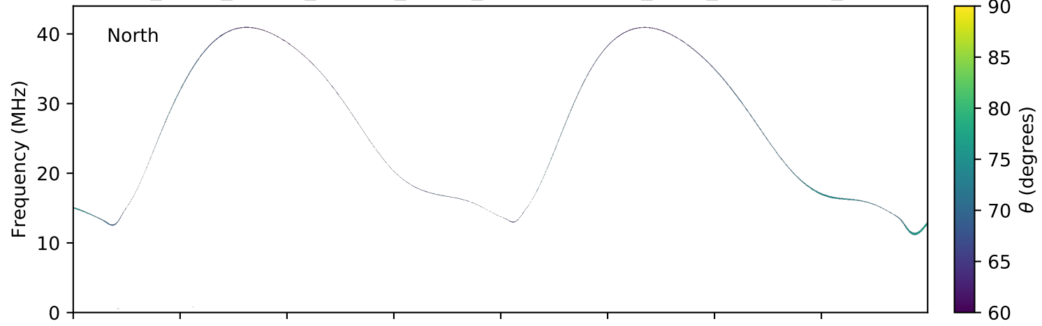
expres_earth_jupiter_europa_jrm09_lossc-wid1deg_3kev_20090428_v01.cdf
