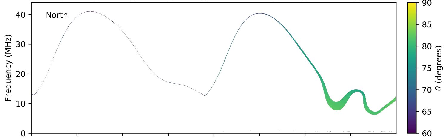
expres_earth_jupiter_europa_jrm09_lossc-wid1deg_3kev_20090414_v01.cdf
