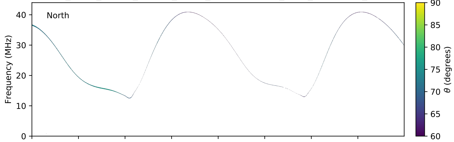
expres_earth_jupiter_europa_jrm09_lossc-wid1deg_3kev_20090410_v01.cdf
