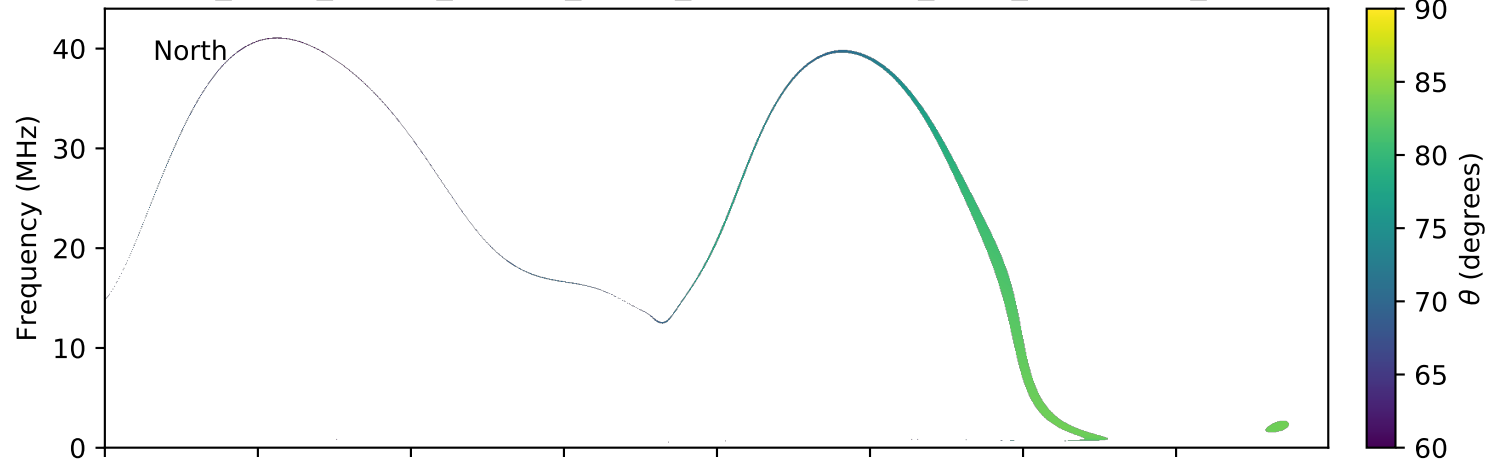
expres_earth_jupiter_europa_jrm09_lossc-wid1deg_3kev_20090407_v01.cdf
