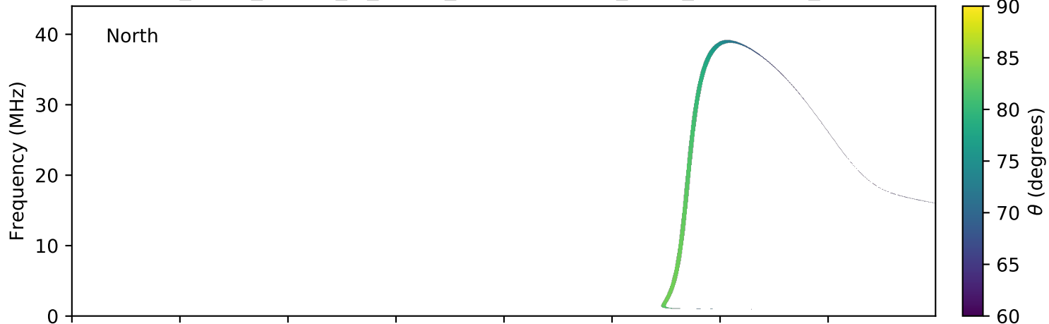
expres_earth_jupiter_io_jrm09_lossc-wid1deg_3kev_20090303_v01.cdf
