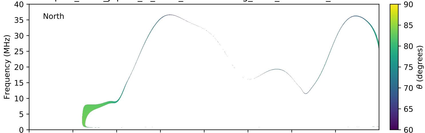
expres_earth_jupiter_io_isaac_lossc-wid1deg_3kev_20090330_v01.cdf
